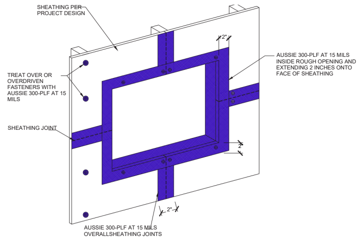
ROUGH OPENINGS - PRETREATMENT METHOD
