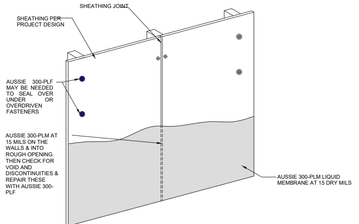
SHEATHING JOINTS - POST TREATMENT METHOD
