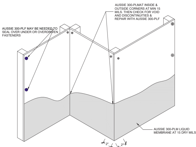
INSIDE CORNERS AND OUTSIDE CORNERS - POST TREATMENT METHOD
