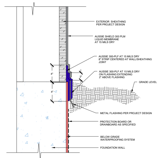
BELOW GRADE TRANSITIONS
