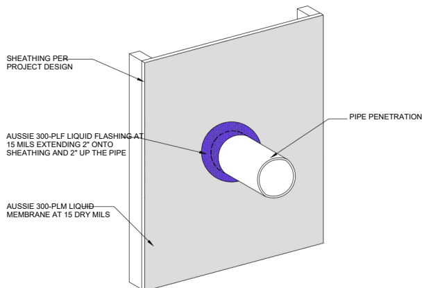
PIPE AND MECHANICAL PENETRATIONS
