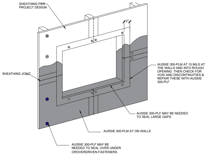
ROUGH OPENINGS - POST TREATMENT METHOD - TYPICAL WINDOW FLASHING NO PRE TREATMENT
