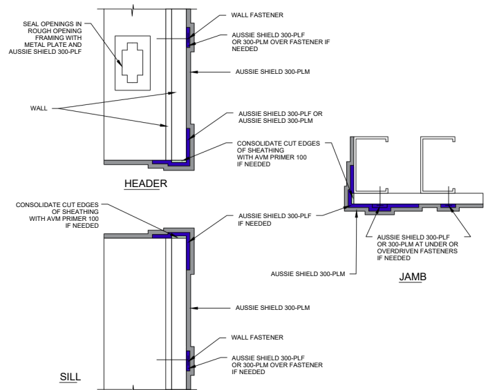
WEB HOLES OR PUNCHOUT REPAIR
