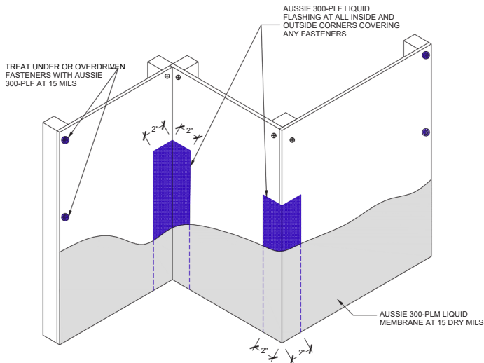
INSIDE AND OUTSIDE CORNERS - PRETREATMENT METHOD
